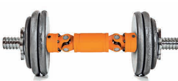
Pure power: Cardan shaft in WANGEN pumps
