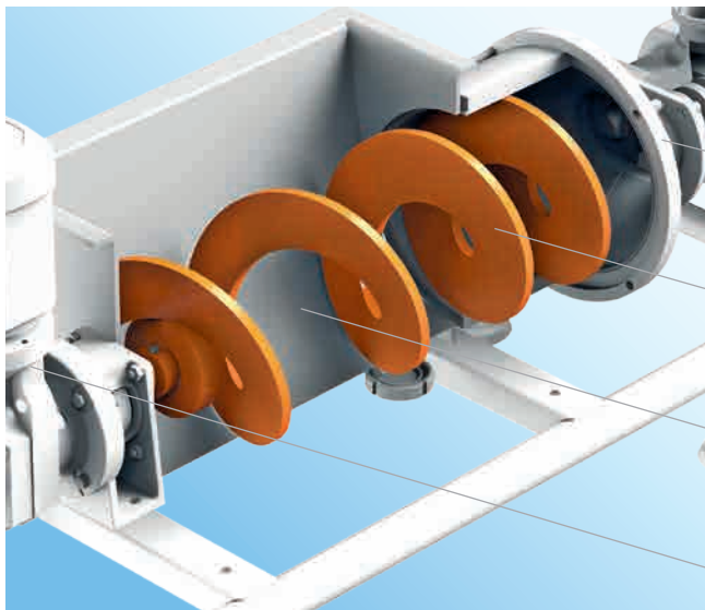
Cross-section of the 'VarioTwin' hopper.
