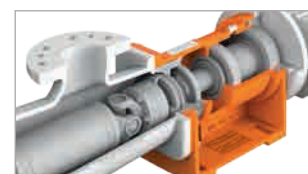
Bearing bracket in KL-S
